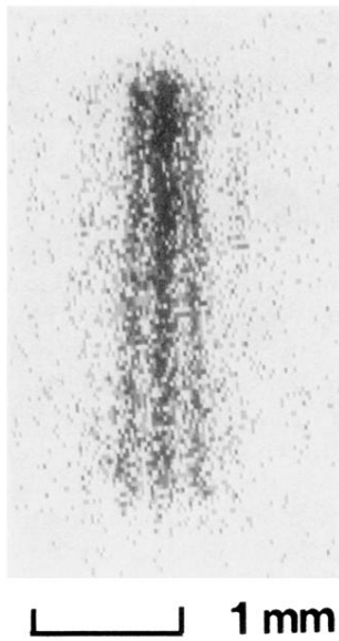
FIG. 2. The interference fringe pattern on the MCP for atoms with the initial velocity of approximately zero. The vertical length of the slit image is 2.8 mm. The spatial resolution of the picture is 20 and 32 \mu\text{m} for the horizontal and vertical directions, respectively. The narrowing of the fringe separation on the upper part is due to the damage of the double-slit structure. This figure contains approximately 6 \times 10^3 atomic counts.
