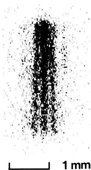
FIG. 2. The interference fringe pattern on the MCP for atoms with the initial velocity of approximately zero. The vertical length of the slit image is 2.8 mm. The spatial resolution of the picture is 20 and 32 \mu\text{m} for the horizontal and vertical directions, respectively. The narrowing of the fringe separation on the upper part is due to the damage of the double-slit structure. This figure contains approximately 6 \times 10^3 atomic counts.
